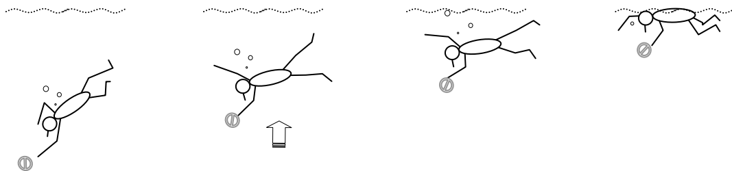
One example of feeling the effect of upthrust. When trying to pick up something from the pool floor, the swimmer will find that he/she will come back to the surface with very little or no effort.
